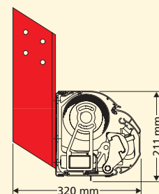
Rafter mounting
