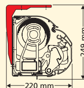
Ceiling mounting
