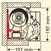
Niche installation
