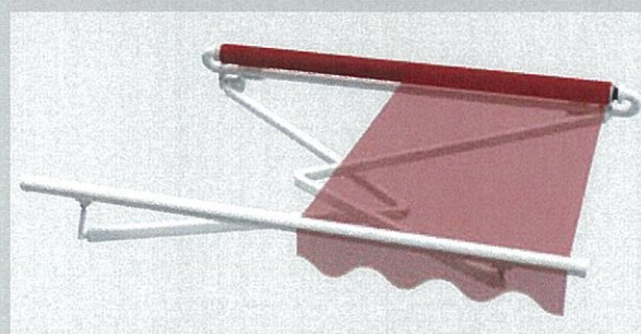
arms cross above one another during extension and retraction, arm fixture to the torque bar and the front profile.
